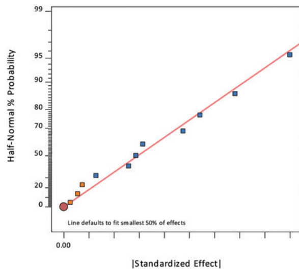
Figure 8: Half-normal Plot of Effects from Ruggedness Test
