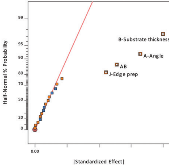
Figure 3: Factors A, B, and J Stand Out for Welding
