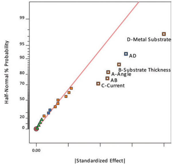
Figure 5: Characterization Study Reveals Interactions between Welding Factors
